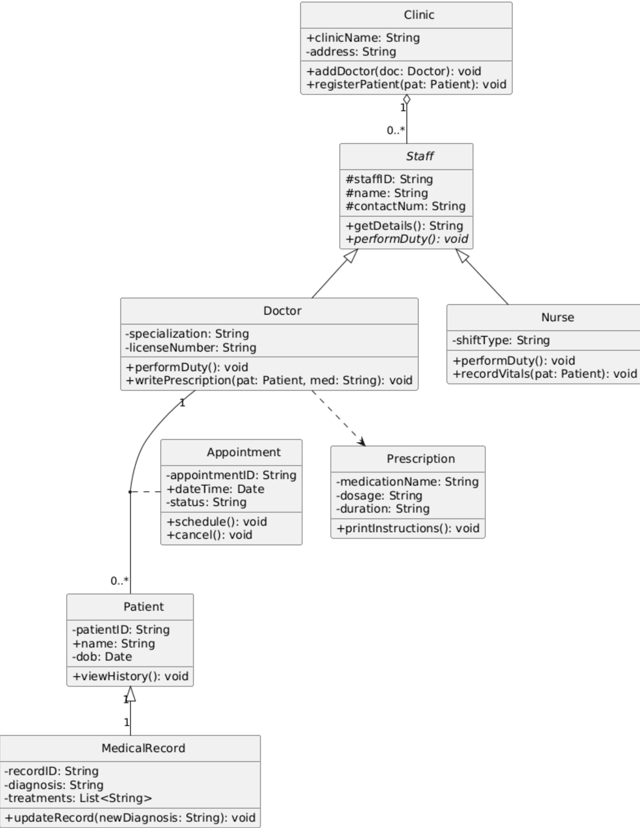
Medical Clinic System - Class Diagram
